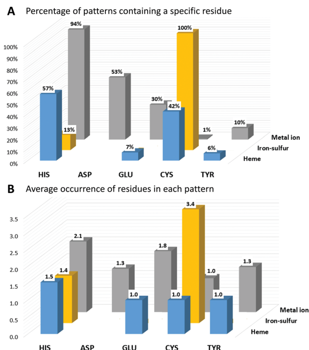
Fig. 1 Analysis of the first coordination sphere for the predicted iron-binding proteins; (A) percentage of patterns containing a specific residue for different iron cofactor types. (B) Average occurrence of a specific residue within patterns, for each iron cofactor.
