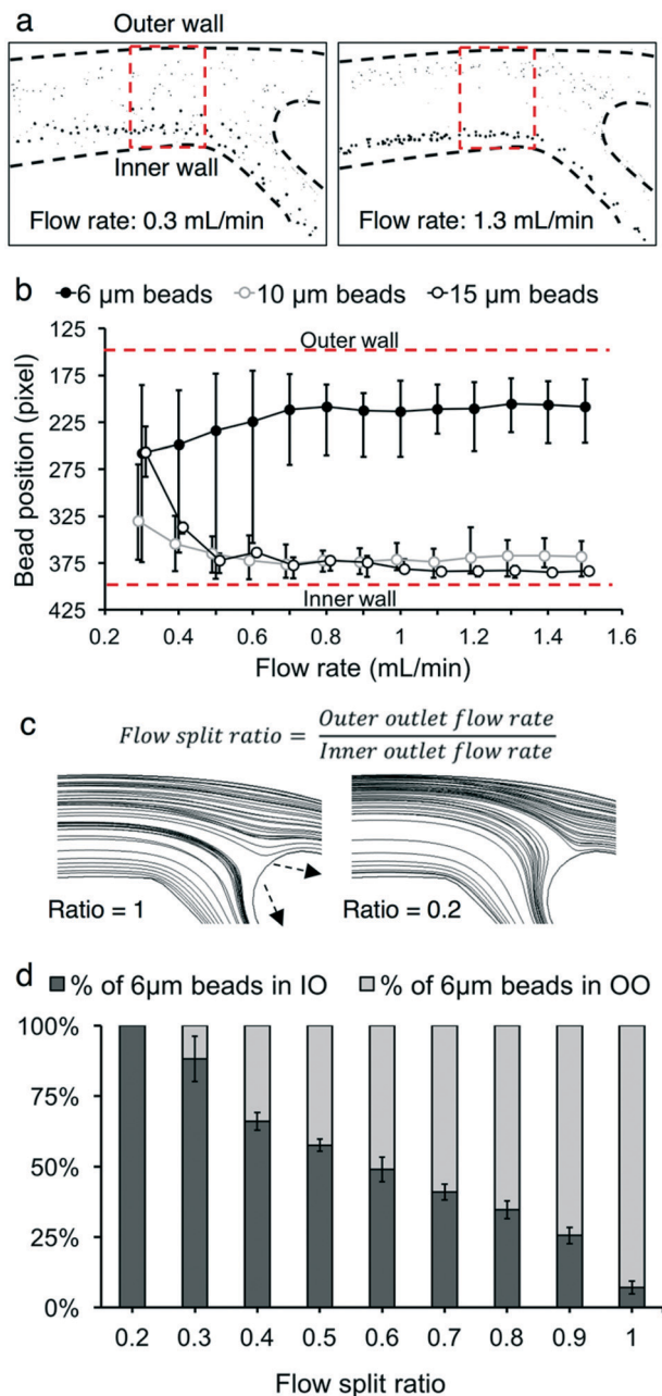
Fig. 3 Device characterization using micro beads. (a) Photographs of 6 μm and 15 μm beads at the bifurcation of the microfluidic device obtained at 0.3 mL min -1 and 1.3 mL min -1 flow rates. (b) Quantification of the bead position at different flow rates. The beads' positions were obtained within the region marked in (a). The flow split ratio was maintained at 0.3 in (a) and (b). Error bars, data range ( n = 3 ). (c) The flow split ratio was defined as the ratio of the outer outlet flow rate to the inner outlet flow rate. This adjusts the flow streamline boundary between flows into the inner and outer outlets. The outlet flow rates were measured based on the amount of fluid that comes out of the outlets per time unit. Tubes with different diameters and lengths modulated the fluidic resistance of the outlets. The streamline boundary at a 0.2 flow split ratio moved closer to the outer wall compared with the boundary at a 1 flow split ratio. (d) The effects of the flow split ratio on the distribution of the 6 μm beads in the inner outlet (IO) and outer outlet (OO) of the microfluidic device. 10 μm and 15 μm beads (not shown) were focused into the inner outlet regardless of the flow split ratio. The flow rate was maintained at 1.0 mL min -1 . Error bars, data range ( n = 3 ).
