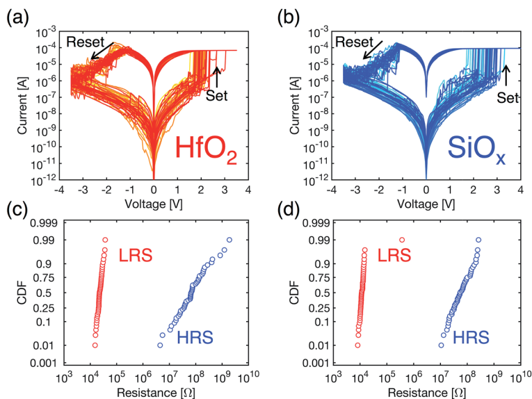
Fig. 4 Measured I - V curves for \text{HfO}_2 (a) and for \text{SiO}_x (b), and the corresponding distributions of resistance for the HRS and LRS (c, d). The compliance current was I_{\text{C}} = 80 \mu\text{A} and the stop voltage was V_{\text{stop}} = -3.5 \text{ V} . The resistance window is about 5000 in both cases, which supports a similar mechanism for switching in the two stacks.
