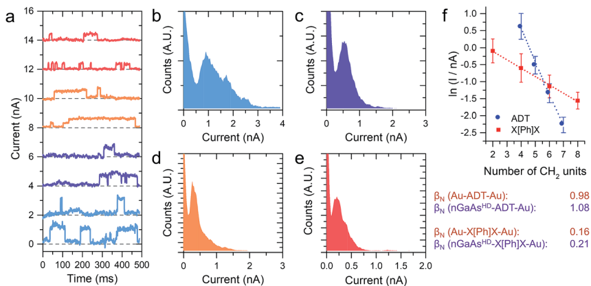
Fig. 3 (a) Example I(t) traces for \text{nGaAs}^{\text{HD}}\text{-X[Ph]X-Au} junctions. Traces are offset on the y axis for clarity. (b) Histogram constructed from 1154 individual current jumps for \text{nGaAs}^{\text{HD}}\text{-1[Ph]1-Au} junctions. (c) Histogram constructed from 532 individual current jumps for \text{nGaAs}^{\text{HD}}\text{-2[Ph]2-Au} junctions. (d) Histogram constructed from 1196 individual current jumps for \text{nGaAs}^{\text{HD}}\text{-3[Ph]3-Au} junctions. (e) Histogram constructed from 970 individual current jumps for \text{nGaAs}^{\text{HD}}\text{-4[Ph]4-Au} junctions. (f) Plot of current jump magnitude versus number of \text{CH}_2 units plot used to determine the value of \beta_N . All data shown in this Figure is obtained in the dark.
