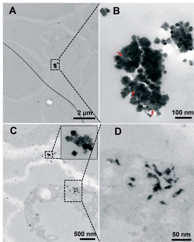
Fig. 1 TEM images of the root sections of soybean treated with \text{nCeO}_2 under the -P condition. (A) and (C) show the intercellular regions. (B) and (D) are the magnified images of the highlighted rectangle areas in A and C. Red arrows in B indicate the \text{nCeO}_2 that were morphologically “transformed”.
