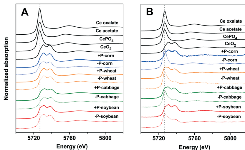
Fig. 2 Ce L-III edge XANES spectra of the root (A) and shoot (B) of the plants with treatment of 2000 \text{ mg L}^{-1} \text{nCeO}_2 for 2 weeks under the +P (solid lines) and -P (dotted lines) conditions. Vertically dotted line indicates the peak of the Ce(III) species centered at 5726.7 eV.
