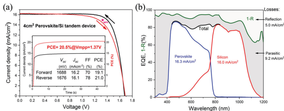
Fig. 7 (a) J–V curve and in the inset: steady-state PCE of the champion tandem device on 4 cm 2 using the heavier p++ front emitter for the Si bottom cell and with antireflection foil on the front of the tandem. (b) EQE for the corresponding device (black), for the perovskite top cell (blue), and for the silicon bottom cell (red). The total absorbance (1-reflectance) of the tandem device is shown by the green line.
