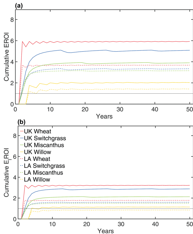
Fig. 4 Dynamic EROI of biomass pellets (top) and dynamic E_{IROI} of abated bioelectricity (bottom) for the two feedstock case studies, in the median scenario. In the case of willow, upon importing pellets as opposed to using domestic pellet, the system becomes energy negative, as the lifetime E_{IROI} is found below one. For energy positive systems, the E_{I}PBT varies from 1 to 4 years.
