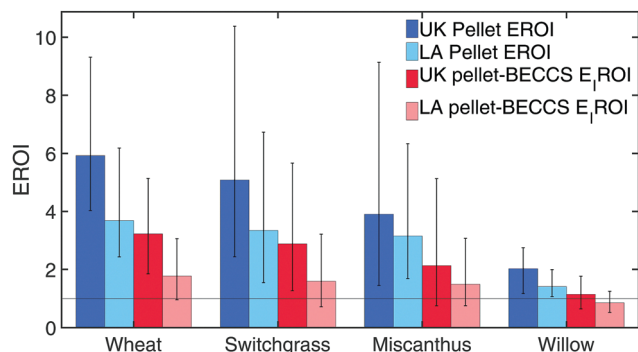
Fig. 5 Lifetime EROI of biomass pellets (blue) and lifetime E_{IROI} of abated bioelectricity (red) for the two case studies. The lifetime cumulative EROI vary from 1.1 to 10.4, whereas the lifetime cumulative E_{IROI} values drop to between 0.5 to 5.7.
