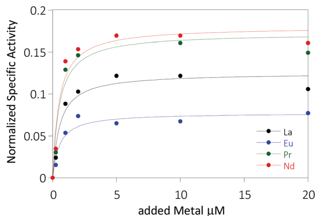
Fig. 2 Normalized specific activity ( n = 3 , for 5 and 10 μM n = 1 ) of 200 nM ‘partial- apo ’ Eu-MDH in the presence of increasing amounts of LnCl 3 , error bars were omitted for clarity, standard deviations from the mean were less than 10%. The data was normalized by subtracting the activity of Eu-MDH without added Ln from the data.
