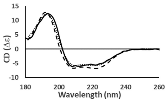
Fig. 7 Comparison of the experimental spectrum (—) and the predicted spectra produced using the PDB2CD 38 (---) and PDCMD2CD 39 (···) servers for the protein calnexin (PDBID 2CCM; PCDDBD CD0004676000).
