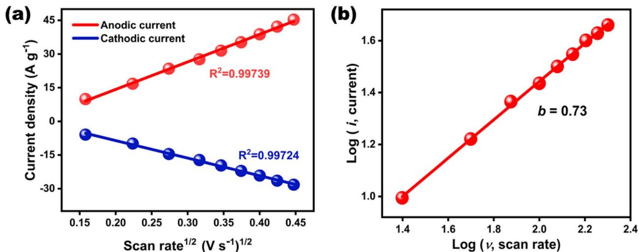
Fig. 7 (a) Cathodic and anodic peak current density ( i_p ) vs. the square root of scan rate ( v^{1/2} ) and (b) plots of \log(i_p) and \log(v) for rGO/MnO 2 .
