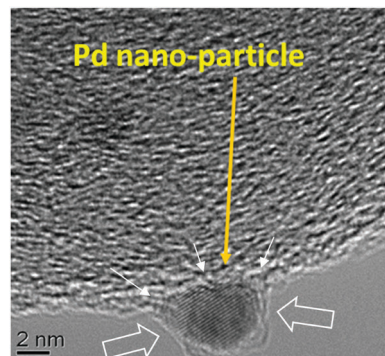
Fig. 28 HRTEM image of a Pd nanoparticle supported over a functionalized CNT. Small arrows indicate new defective areas created at the carbon–nanoparticle interfaces, while large arrows indicate carbon shells wrapping the nanoparticle.
