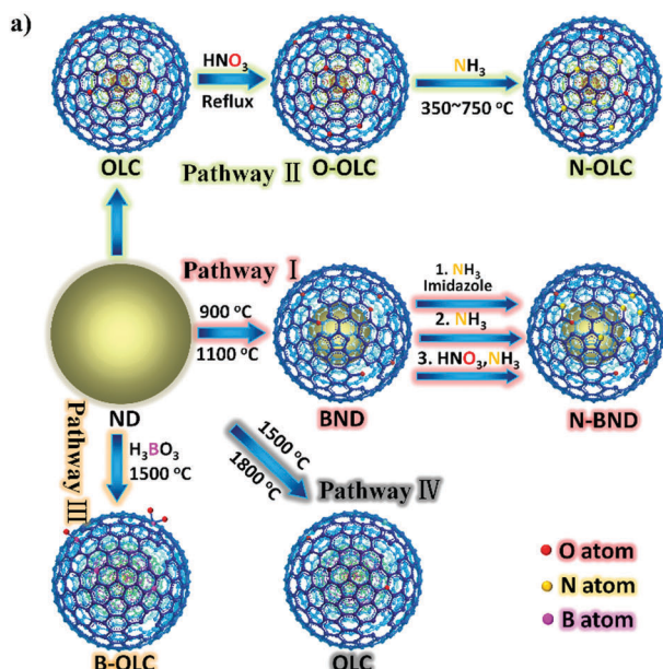
Fig. 8 (a) Sketch for the production of UNDDs and related materials. (b) The possible evolution pathways of different nitrogen species during the preparation process of nitrogen-modified UNDDs (two hexatomic rings as ideal starting model structures in different pathways). Reproduced from ref. 156 with permission from American Chemical Society, copyright 2014.
