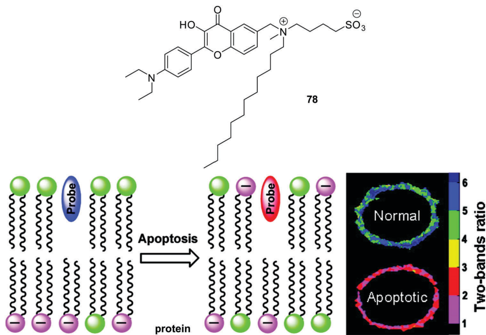
Scheme 67 A dodecyl functionalised 3-hydroxyflavone probe 78. This system is incorporated into cell membranes and may be used to monitor changes in the lipid membrane content during the early stages of apoptosis. Measurement conditions: lipid. Adapted with permission from ( J. Am. Chem. Soc. , 2007, 129 , 2187–2193). Copyright (2007) American Chemical Society.
