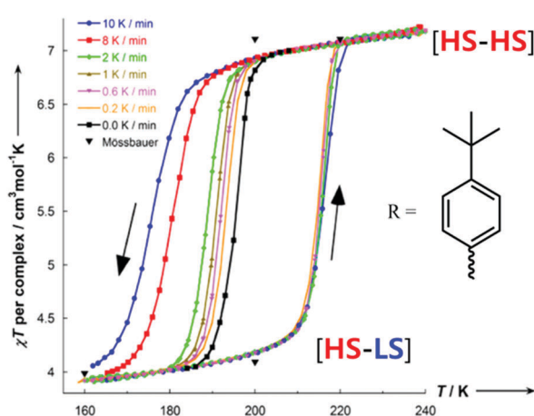
Fig. 13 Scan rate dependence of the thermal hysteresis loop of [\text{Fe}_2^{\text{II}}(\text{PM}^{\text{t-BuPhT}})_2](\text{BF}_4)_4 \cdot 3\frac{1}{2}\text{H}_2\text{O} . Figure adapted with permission from ref. 85. Copyright 2014 ACS.
