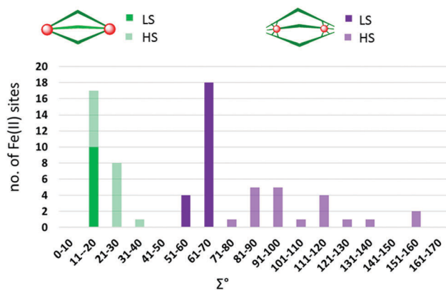
Fig. 55 Distribution of octahedral distortion parameter, \Sigma (°), for the Fe(II) centres in dinuclear complexes of type 2A (Fig. 2): triply triazole bridged [Fe 2 L 5 (NCE) 4 ] (green) and triple helicates [Fe 2 L 3 ] (violet). Dark colour = LS; light colour = HS.
