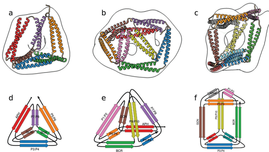
Fig. 3 Model structure of representative CCPO cages in the shape of a (a) tetrahedron, (b) square pyramid and (c) trigonal prism, respectively composed of 12, 16 or 18 CC dimers, obtained from SAXS analysis and superimposed to volumes obtained by EM negative stain single-particle reconstruction. 21 (d–f) Respective schemes; CC segments are represented as colored arrows.
