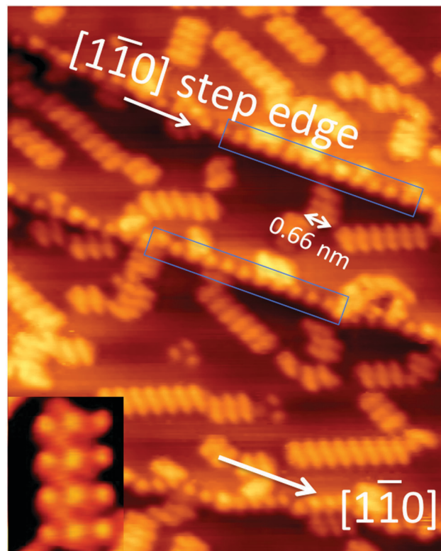
Fig. 1 STM image, 15 nm \times 20 nm, acquired at 77 K from Au(111) with 0.2 ML of methylthiolate. The two blue rectangular boxes highlight two segments of [1\bar{1}0] oriented step edges. The inset shows a high-resolution image where two \text{CH}_3 groups and their associated Au adatoms in each staple are resolved.
