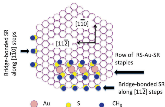
Fig. 3 Structural model illustrating how SCH 3 is bonded to Au atoms along step edges. Along the [112] step, there are two bridging sites available for each SCH 3 . Binding of SCH 3 at one of the bridging sites may be more favorable than the other. In the figure, SCH 3 is placed arbitrarily at one of the bridging sites.
