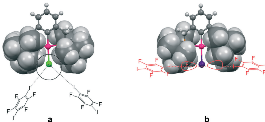
Fig. 10 The tert -butyl fragment of a (2,6-bis[(di- t -butylphosphino)methyl]phenyl) \text{PdX} (ref. 6) ( \text{X} = \text{Cl} (a) and \text{I} (b)) complex is shown as a space filling model to demonstrate the shielding of the 5p equatorial "belt" of the iodide ligand (b), as compared to the spherical chloride "anion" (a), escaping the shield.
