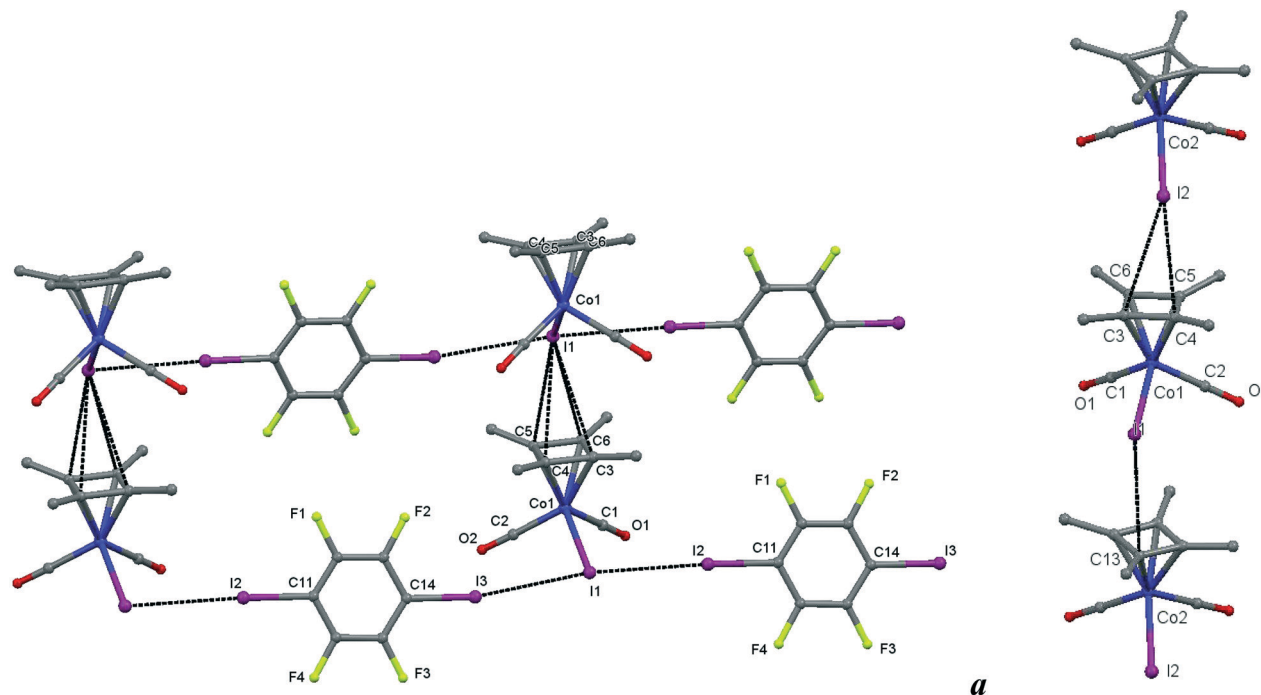
Fig. 8 a) Crystal structure diagram of 6 , showing a fragment of I-I halogen-bonded polymeric chains [\text{Cb}^*\text{Co}(\text{CO})_2][\mu_2\text{-DITFB}]_n linked by \text{I}-\pi(\eta_4\text{-Me}_4\text{C}_4) interactions. Hydrogen atoms are omitted for clarity. Selected distances (Å): intramolecular \text{Co}(1)-\text{I}(1) , 2.619(1); intermolecular \text{I}(3)-\text{I}(1) , 3.589(1); \text{I}(1)-\text{I}(2) , 3.585(1); \text{I}(1)-\text{C}(3-6) ring of the \eta^4 = \text{Me}_4\text{C}_4 ligand, 3.781(7)–3.866(7). Selected angles ( ^\circ ): \text{I}(3)-\text{I}(1)-\text{I}(2) , 171.51(2); \text{Co}(1)-\text{I}(1)-\text{I}(3) , 93.00(2); \text{Co}(1)-\text{I}(1)-\text{I}(2) , 95.16(2); \text{C}(14)-\text{I}(3)-\text{I}(1) , 169.6(2); \text{C}(11)-\text{I}(2)-\text{I}(1) , 177.2(2). b) Comparison of the \text{Cb}^*\text{Co}(\text{CO})_2 stacks in 6 with those in the parent crystal. Selected distances (Å): intermolecular \text{I}(2)-\text{C}(4) , 3.725(8); \text{I}(2)-\text{C}(3) , 3.87(1); \text{I}(1)-\text{C}(13) , 3.842(9), and similarities of the intramolecular distances \text{Co}(2)-\text{I}(2) , 2.598(1); \text{Co}(1)-\text{C}(2) , 1.781(7); \text{C}(2)-\text{O}(2) , 1.157(9); \text{Co}(1)-\text{C}(1) , 1.79(1); \text{C}(1)-\text{O}(1) , 1.16(1). Dotted lines link specific atoms at a distance shorter than the sum of their vdW radii. 18
