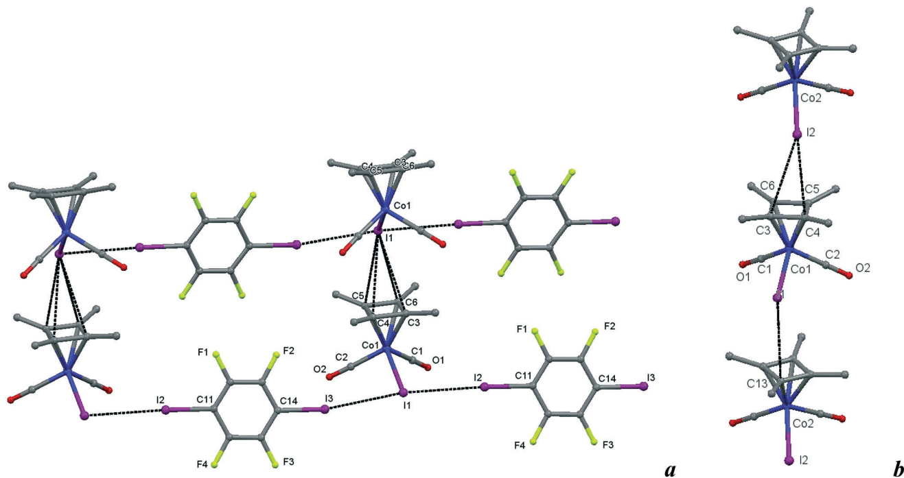
Fig. 8 a) Crystal structure diagram of 6 , showing a fragment of I-I halogen-bonded polymeric chains [\text{Cb}^*\text{Co}(\text{CO})_2][\mu_2\text{-DITFB}]_n linked by \text{I}-\pi(\eta_4\text{-Me}_4\text{C}_4) interactions. Hydrogen atoms are omitted for clarity. Selected distances (Å): intramolecular \text{Co}(1)-\text{I}(1) , 2.619(1); intermolecular \text{I}(3)-\text{I}(1) , 3.589(1); \text{I}(1)-\text{I}(2) , 3.585(1); \text{I}(1)-\text{C}(3-6) ring of the \eta^4 = \text{Me}_4\text{C}_4 ligand, 3.781(7)–3.866(7). Selected angles ( ^\circ ): \text{I}(3)-\text{I}(1)-\text{I}(2) , 171.51(2); \text{Co}(1)-\text{I}(1)-\text{I}(3) , 93.00(2); \text{Co}(1)-\text{I}(1)-\text{I}(2) , 95.16(2); \text{C}(14)-\text{I}(3)-\text{I}(1) , 169.6(2); \text{C}(11)-\text{I}(2)-\text{I}(1) , 177.2(2). b) Comparison of the \text{Cb}^*\text{Co}(\text{CO})_2 stacks in 6 with those in the parent crystal. Selected distances (Å): intermolecular \text{I}(2)-\text{C}(4) , 3.725(8); \text{I}(2)-\text{C}(3) , 3.87(1); \text{I}(1)-\text{C}(13) , 3.842(9), and similarities of the intramolecular distances \text{Co}(2)-\text{I}(2) , 2.598(1); \text{Co}(1)-\text{C}(2) , 1.781(7); \text{C}(2)-\text{O}(2) , 1.157(9); \text{Co}(1)-\text{C}(1) , 1.79(1); \text{C}(1)-\text{O}(1) , 1.16(1). Dotted lines link specific atoms at a distance shorter than the sum of their vdW radii. 18
