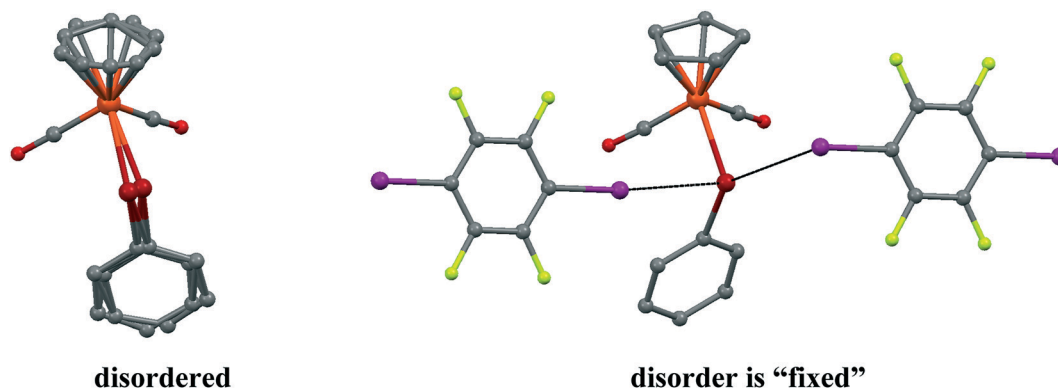
Fig. 3 The disorder of CpFe(CO) 2 TePh molecules in a parent crystal (LADWOE 19 ) is “fixed” by two p -DITFB molecules in cocrystal 1.
