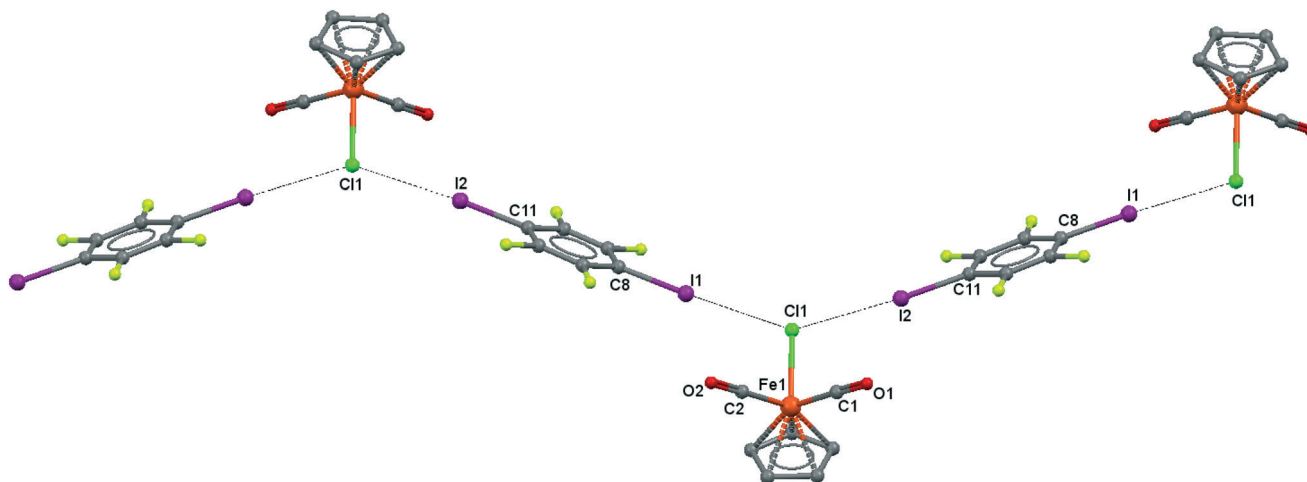
Fig. 5 Crystal structure diagram of 3, showing a fragment of I–Cl halogen-bonded polymeric chains ([CpFe(CO) 2 Cl](μ 2 -DITFB)) n . Hydrogen atoms are omitted for clarity. Selected distances (Å): Fe(1)–Cl(1), 2.318(3); Cl(1)–I(1), 3.219(5); Cl(1)–I(2), 3.229(5). Selected angles (°): I(2)–Cl(1)–I(1), 141.48(3); Fe(1)–Cl(1)–I(1), 110.02(4); Fe(1)–Cl(1)–I(2), 108.33(4); Cl(1)–I(2)–C(11), 173.4(1); Cl(1)–I(1)–C(8), 175.8(1). Dotted lines link Cl and I atoms at distances shorter than the sum of Cl–I vdW radii. 18
