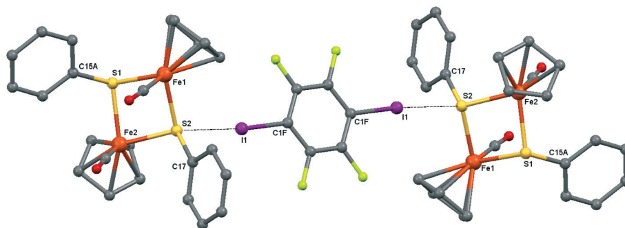
Fig. 4 Crystal structure diagram of 2, showing its I–S halogen-bonded trimolecular assemblies ([CpFe(CO)(μ 2 -SPh)] 2 (μ 2 -DITFB)). Hydrogen atoms are omitted for clarity. Selected distances (Å): I(1)–S(2), 3.130(1). Selected angles (°): C(1F)–I(1)–S(2), 173.9(1); Fe(1)–S(2)–I(1), 111.91(4); I(1)–S(2)–C(17), 102.5(1); I(1)–S(2)–Fe(2), 118.86(4). Dotted lines link S and I atoms at a distance shorter than the sum of the S–I vdW radii. 18
