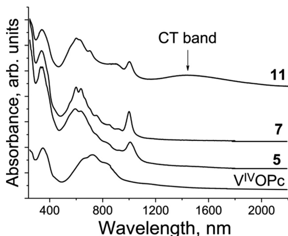
Fig. 15 Spectra of pristine \text{V}^{\text{IV}}\text{O}(\text{Pc}^{2-}) and selected salts 5, 7 and 11 in the UV-visible-NIR ranges in KBr pellets. Pellets for the salts were prepared under anaerobic conditions.
