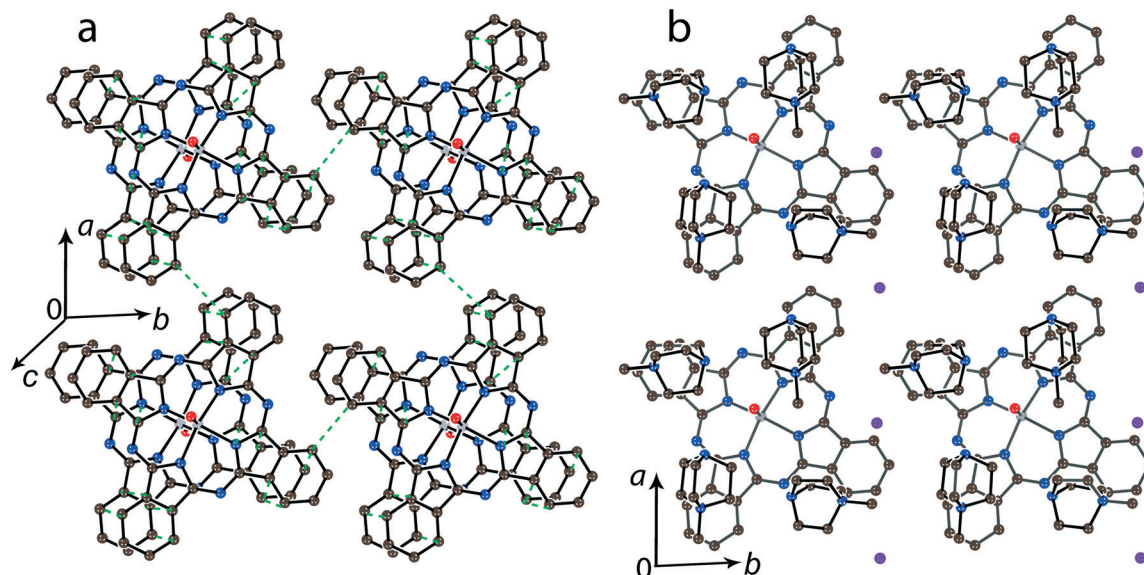
Fig. 8 (a) View of the phthalocyanine layer composed of the \pi -stacking [\{\text{Ti}^{\text{IV}}\text{O}(\text{Pc}^{3-})\}]_2 dimers in 13 . Short van der Waals C...C, N...C contacts are shown by green dashed lines. (b) Projection of the (\text{MDABCO})_2^+ layer on the phthalocyanine layer. Only one phthalocyanine from the dimer is shown (bonds are shown in grey). Salt 14 is isostructural to 13 .
