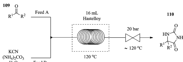
Fig. 15 Continuous flow synthesis of hydantoin.
