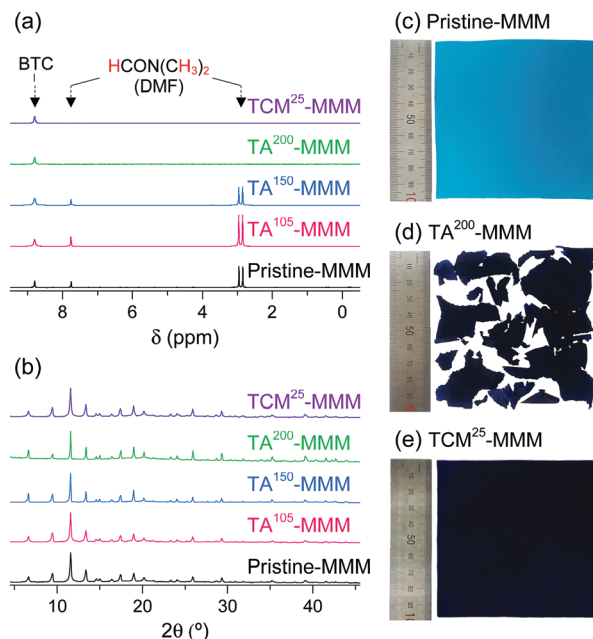
Fig. 18 (a) 1 H NMR spectra and (b) PXRD patterns of pristine-, TA 105 -, TA 150 -, TA 200 -, and TCM 25 -MMM. Photographs of (c) pristine-MMM, (d) TA 200 -MMM, and (e) TCM 25 -MMM. Reprinted (adapted) with permission from ref. 70. Copyright (2018) American Chemical Society.
