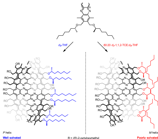
Fig. 7 Suginome's screw-sense switching in poly(quinaxaline-2,3-diyl)s.
