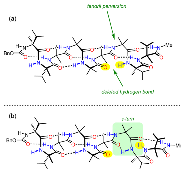
Fig. 12 (a) Tendrils perversions and (b) \gamma -turns in Aib foldamers.
