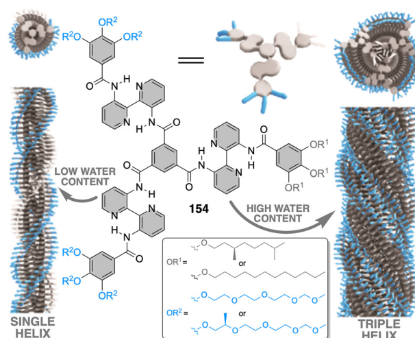
Fig. 75 Chemical structure of amphiphilic BiPy-BTA (154) and its hierarchical self-assembly from supramolecular fibre to triple helical bundle depending on the water content of water-isopropanol mixtures. Reproduced from ref. 365 with permission from the American Chemical Society, copyright 2014.
