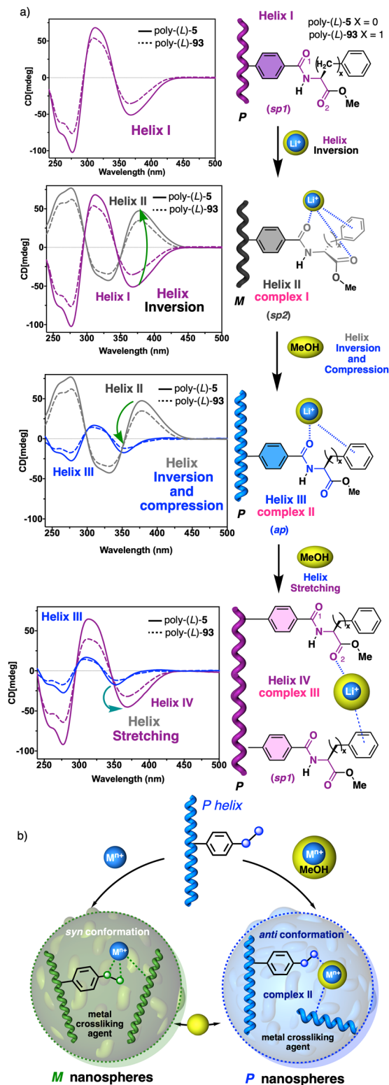
Fig. 40 (a) Elongation and helical sense control via dynamic coordination chemistry in poly-(L)-5 and poly-(L)-93/ Li^+ /MeOH complexes. (b) Illustration of nanostructuring via dynamic coordination chemistry. Reproduced from ref. 229 with permission from the Royal Society of Chemistry, copyright 2017.
