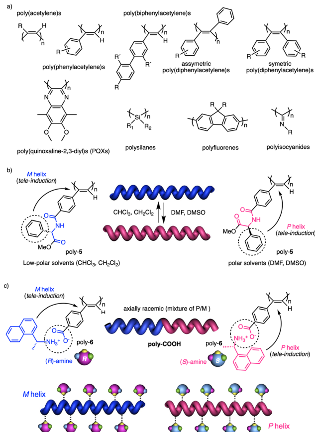
Fig. 2 (a) Some families of dynamic helical polymers. (b) Helix inversion of a chiral poly(phenylacetylene) bearing 4-benzamide of (S)-phenylglycine methyl ester as pendant group by tuning its conformational composition using solvent polarity as external stimulus. (c) Chiral amplification of an achiral poly(phenylacetylene) bearing 4-benzoic acid as pendant using chiral amines as external stimuli.
