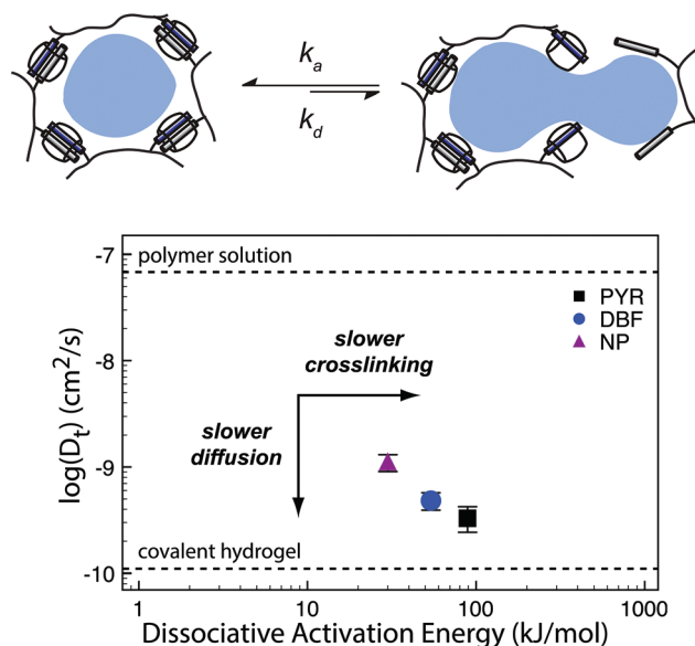
Fig. 10 (a) Supramolecular hydrogels that use non-covalent crosslinks, such as the CB[8] ternary complexes shown above, exhibit time-dependent mesh sizes that depend on the kinetics of the crosslink interactions. These hydrogels can exhibit identical crosslink thermodynamics, but varying kinetics due to the different guest moieties. (b) A supramolecular interaction can have different dissociation kinetics, but similar binding thermodynamics. Using the example of hydrogels prepared with CB[8] ternary complex crosslinks with data adapted from ref. 175 we demonstrate that different diffusion profiles for the same cargo are achieved for materials of similar moduli due to varying guest moieties (PYR = pyrone (slow); DBF = dibenzofuran (medium); Np = naphthalene (fast)). Moreover, scattering experiments illustrated that these gels were isostructural.
