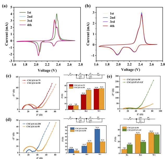
Fig. 8 (a) CV curves of CSC@S/Al cells with 50 \mu m thickness (b) CV curves of CSC@S/PAN-GF cells (c) different electrodes Nyquist curves and equivalent circuit parameters of electrodes (c) CSC@S/Al-50 and CSC@S/Al-75 (d) CSC@S/Al-50 and CSC@S/Al-250 (e) CSC@S/Al-50 and CSC@S/PAN-GF.
