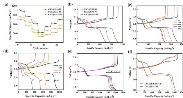
Fig. 5 (a) Rate capability of CSC@S/Al cathode with 50 μm, 75 μm and 250 μm thicknesses charge–discharge cycles of (b) CSC@S/Al cathode with 50 μm, 75 μm and 250 μm thicknesses. (c) CSC@S/Al-50 cathode for 100 cycle (d) CSC@S/Al-50 cathode at 0.2C, 0.5C, 1C and 2C, respectively (e) the first five charge/discharge cycles of CSC@S/Al-50 cathode at 0.1C (f) CSC@S/PAN-GF with CSC@S/Al-50 cathode at 0.1C.
