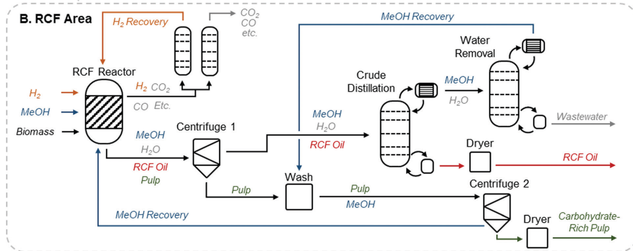
Fig. 1 RCF biorefinery design. (A) Block flow diagram of an RCF-based cellulosic ethanol biorefinery. This process follows a configuration similar to that described by Humbird et al. , with the dilute-acid pretreatment area replaced with RCF. The RCF area produces a lignin-rich RCF oil as a co-product and a carbohydrate-rich pulp. Carbohydrate pulp, the residual biomass solids after the lignin is removed during RCF, is isolated and saccharified to C 5 and C 6 sugars via enzymatic hydrolysis, fermented to ethanol, and recovered to produce fuel-grade ethanol. WWT is the wastewater treatment area. CHP is the combined heat and power area where a combination of natural gas, sludge from WWT, and residual solids from ethanol production are burned to generate steam for process heat and electricity. Excess electricity is sold to the grid as a co-product. (B) The process diagram highlighting major unit operations in the RCF area of the biorefinery for the methanol case. The solvent pump-around RCF reactor design is shown in Fig. S2 (ESI†). The gaseous products are sent to a PSA unit to recover H 2 to be recycled to the reactor, and the liquid and solid products are separated via centrifugation to isolate dilute RCF oil, which is concentrated in a crude distillation column, and water is removed from methanol in the water removal distillation column. After washing with methanol to recover additional lignin oil, the carbohydrate-rich pulp is isolated via a second centrifuge and the methanol rinse is recycled back to the RCF reactor. Major heating and cooling duties were heat integrated to reduce overall energy demand. A process flow diagram with labeled streams and a corresponding table of stream compositions is included in Fig. S1 and Table S2 (ESI†).
