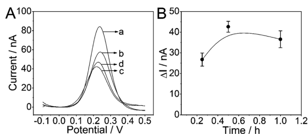
Fig. 4 Electrochemical signal and calibration plot of the Pt \mu E/MoS 2 /Au micro-biosensors: (A) SWV curve of the Pt \mu E/MoS 2 /Au electrodes incubated with 10 -7 M probe DNA for (a) 0 M, (b) 0.25 h, (c) 0.5 h, and (d) 1 h; (B) SWV calibration plot of Pt \mu E/MoS 2 /Au electrodes incubated with 10 -7 M probe DNA for different time range from 0.25 h to 1 h.
