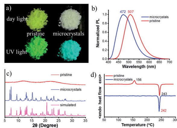
Fig. 2 (a) Photographs of the pristine sample and microcrystals of 1 under day light and UV irradiation (365 nm). (b) Normalized PL spectra of the pristine sample and microcrystals. (c) XRD patterns of the pristine sample, and microcrystals and the simulated pattern of single crystals. (d) DSC thermograms of the pristine sample and microcrystals.
