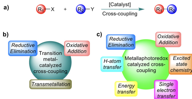
Scheme 1 (a) General scope of C–C coupling reactions. (b) General scheme outlining the elementary steps of ground state transition metal-catalysed C–C cross-coupling. (c) General scheme outlining the elementary steps available for metallaphotoredox-catalysed C–C cross-coupling.
