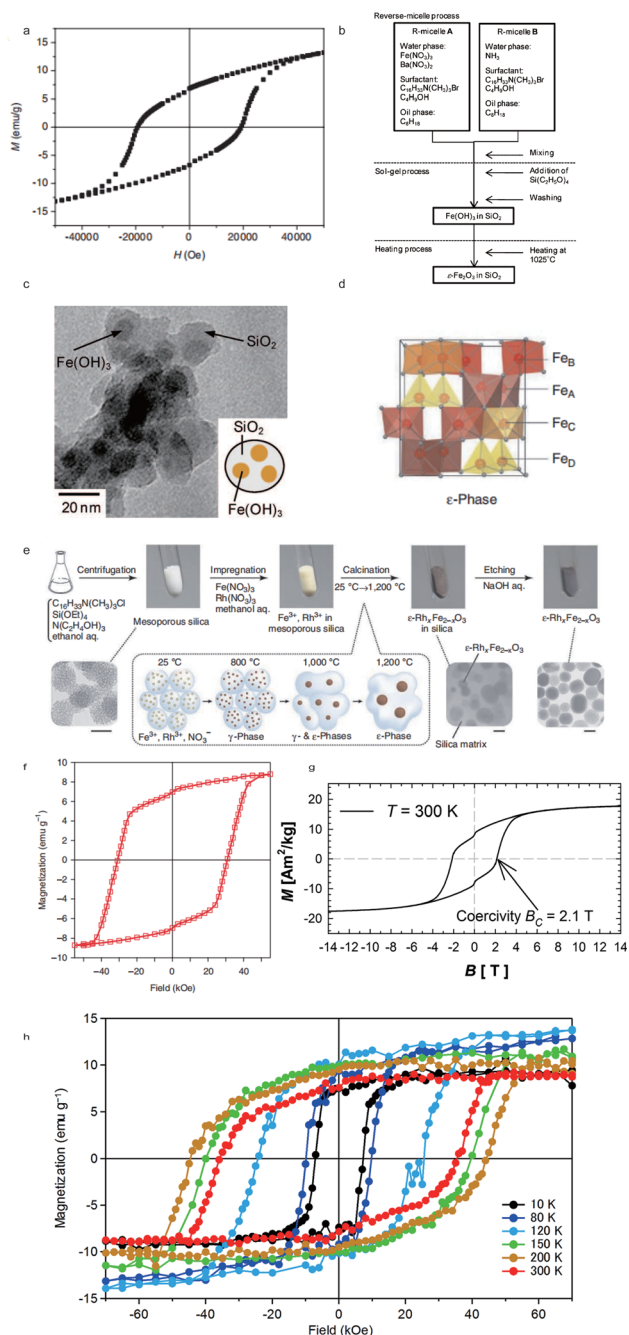
Fig. 6 (a) Magnetic hysteresis loops of \epsilon - \text{Fe}_2\text{O}_3 prepared by Jin et al. ; (b) procedure to prepare SiO 2 -coated \epsilon - \text{Fe}_2\text{O}_3 nanorods; (c) TEM image of \epsilon - \text{Fe}_2\text{O}_3 ; (d) crystal structure of the \epsilon -phase; (e) schematic illustration of synthesis of \epsilon - \text{Fe}_2\text{O}_3 on a silica template; (f) magnetic hysteresis loops of oriented \epsilon - \text{Fe}_2\text{O}_3 at 300 K; (g) magnetic hysteresis loops of powdered \epsilon - \text{Fe}_2\text{O}_3 embedded in a silica matrix at 300 K; (h) magnetic hysteresis loops of \epsilon - \text{Fe}_2\text{O}_3 oriented at different temperatures. Reproduced from ref. 75, 76, 77, 78 and 79 with the permission of John Wiley and Sons, Springer Nature, and AIP Publishing.
