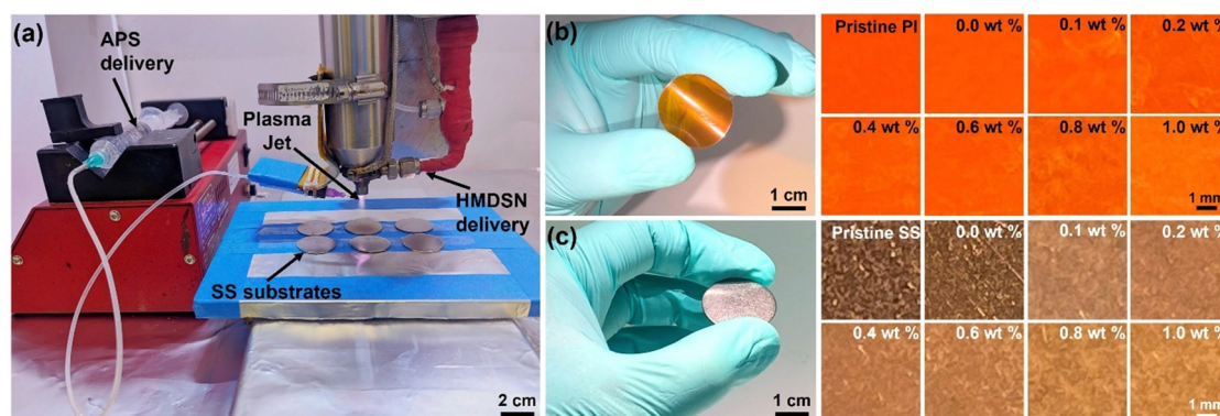
Fig. 2 Plasma assisted deposition of the \text{SiO}_x coating onto PI and SS surfaces with varying APS concentration. (a) Image of the application of the CAP system with two inlets for the silica precursor and APS delivery into the plasma jet. Photographs of (b) PI and (c) 304 SS, with zoomed areas of various samples. Images show the surfaces of the pristine substrate, and the surfaces coated with silica coatings from the precursor containing 0 to 1.0\text{ wt}\% APS.
