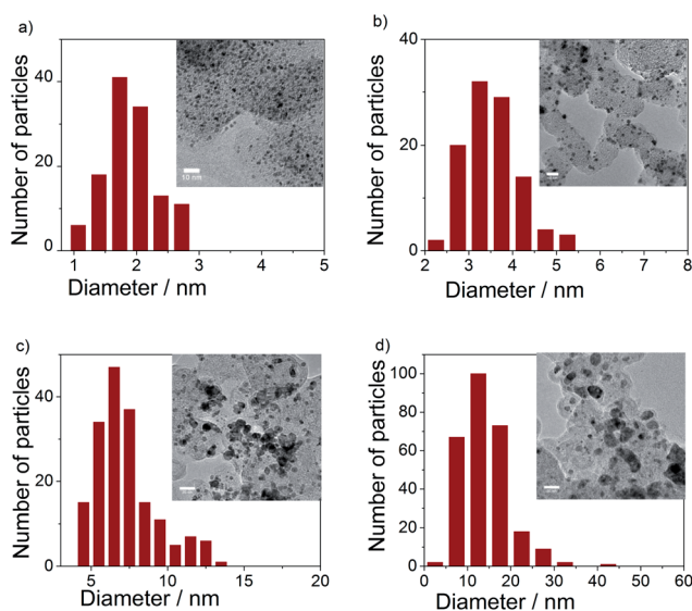
Fig. 3 TEM images and particle size histograms of (a) Ir, (b) IrNi 2.3 , (c) IrNi 3.3 , and (d) IrNi 5.7 precursor alloys.
