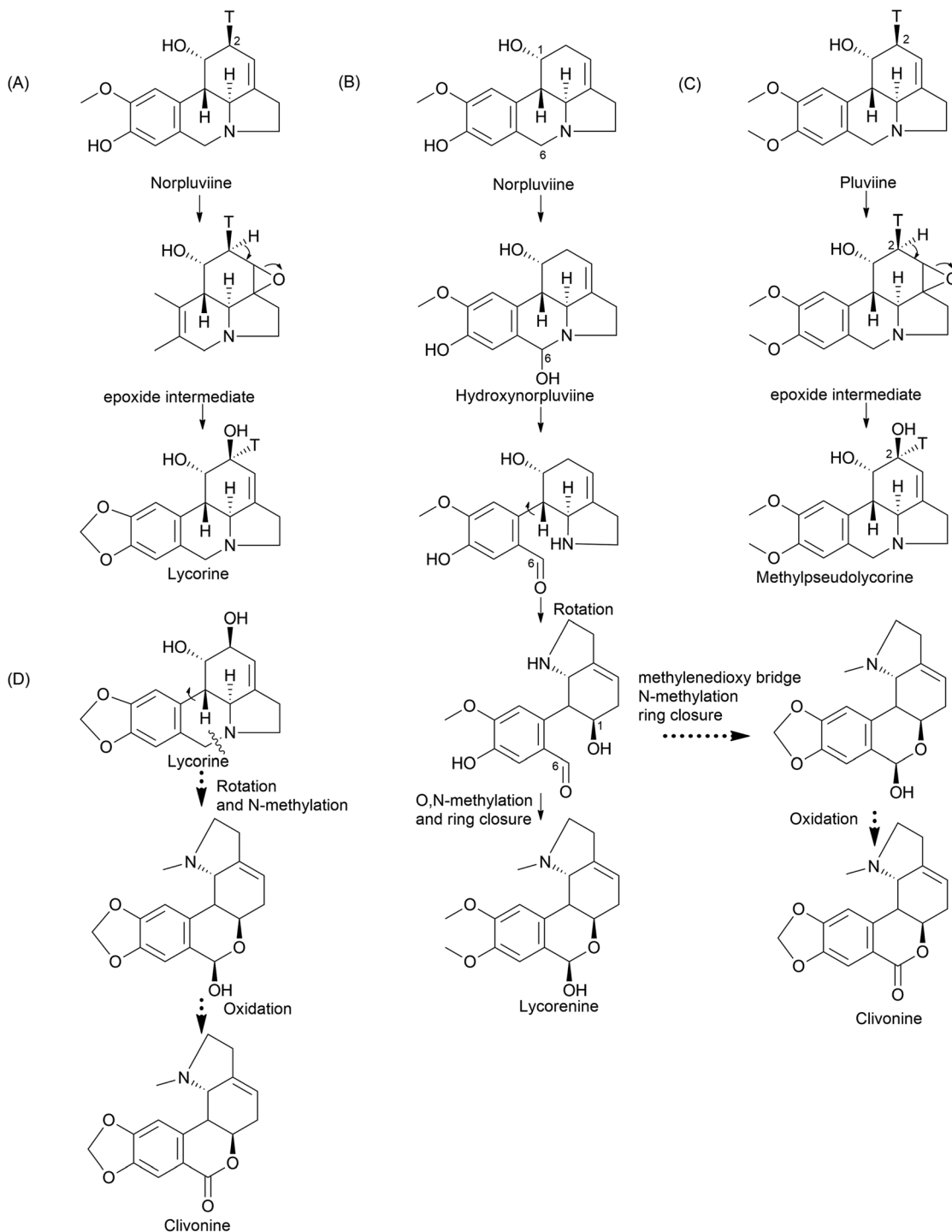
Fig. 8 Ortho-para coupling pathway-related components biosynthetic mechanisms. Norpluviine proceeds to lycorine through (A) inversion and/or retention of C2 tritium elucidates hydroxylation stereospecificity; (B) bond cleavage, rotation, and hemiacetal bond establishment, and another pathway to reach clivonine; (C) suggested epoxide intermediate formation to achieve methylpseudolycorine; (D) clivonine biosynthesis via lycorine.
