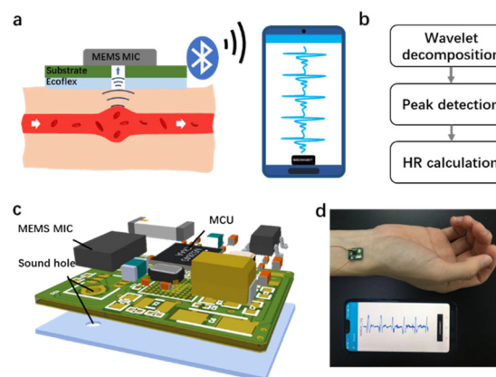
Fig. 1 Design and demonstration of the WSES. (a) Schematics of HR monitoring by our device. (b) Flow chart of signal processing. (c) Design of the device with a PCB and adhesives. (d) Photo of the WSES monitoring HR.
