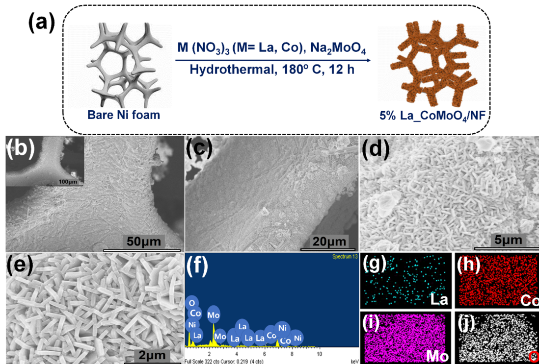
Fig. 1 (a) Schematic representation of the preparation of La-doped CoMoO 4 , (b–e) SEM images of the as-synthesized 5% La-CoMoO 4 , (f–j) corresponding EDS spectrum and elemental mapping analyses of elements La, Co, Mo, and O.
