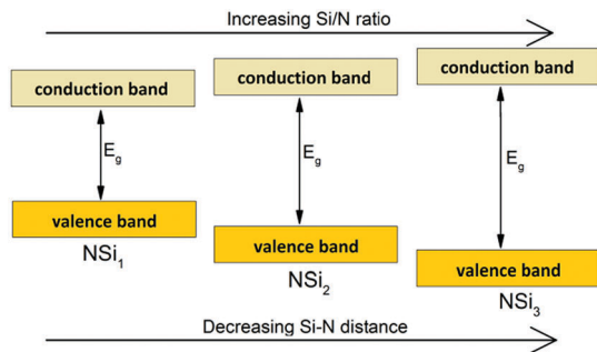
Fig. 7 Schematic diagram, showing the influence of the degree of condensation (Si/N ratio) on the positions of the valence and conduction bands and the size of the bandgap E_g .
