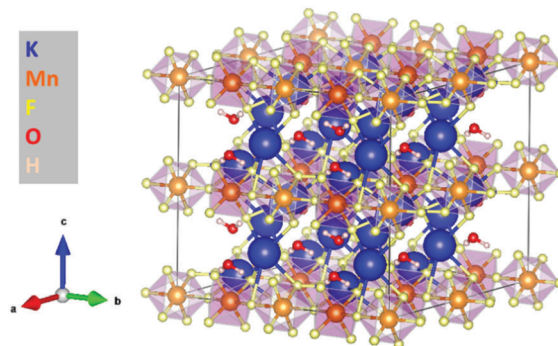
Fig. 7 Structure of the \text{K}_2\text{MnF}_5\cdot\text{H}_2\text{O} hydrate formed during synthesis.
