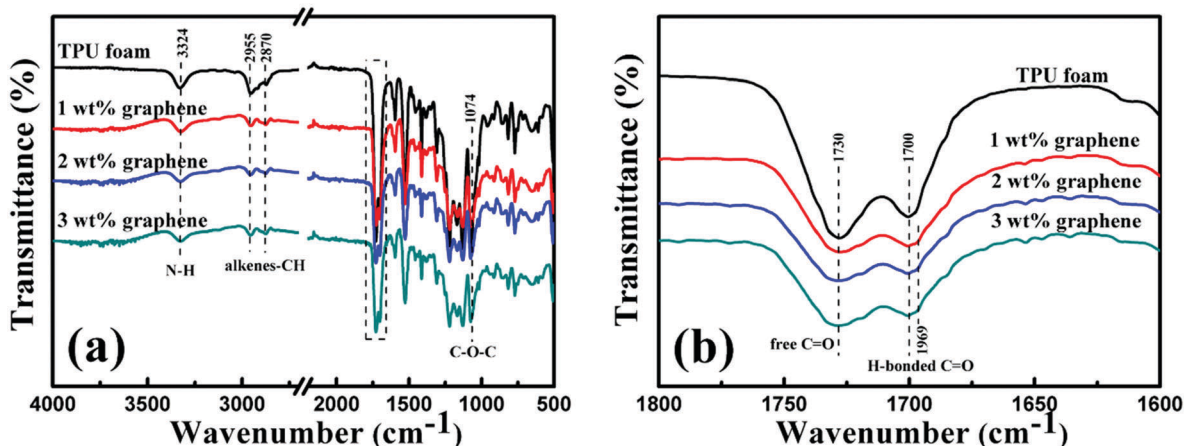
Fig. 5 (a) FT-IR spectra of the TPU foam and its CPC foams with graphene loadings of 1, 2 and 3 wt%. Details of the rectangular area are depicted in (b).
