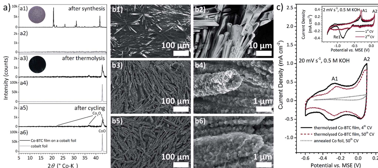
Fig. 1 (a) XRD patterns and photographs (inset a1, a3) of (a1) an electrodeposited [\text{Co}_3(\text{BTC})_2(\text{H}_2\text{O})_{12}] film on Co foil, (a2) Co foil, (a3) a thermolysed [\text{Co}_3(\text{BTC})_2(\text{H}_2\text{O})_{12}] film on Co foil, (a4) a thermally treated Co foil, (a5) a thermolysed [\text{Co}_3(\text{BTC})_2(\text{H}_2\text{O})_{12}] film after CV experiments in 0.5 M KOH on Co foil, (a6) a thermally treated Co foil, (b) SEM images of (b1, b2) an electrodeposited [\text{Co}_3(\text{BTC})_2(\text{H}_2\text{O})_{12}] film, (b3, b4) a thermolysed [\text{Co}_3(\text{BTC})_2(\text{H}_2\text{O})_{12}] film, (b5, b6) a thermolysed [\text{Co}_3(\text{BTC})_2(\text{H}_2\text{O})_{12}] film after CV experiments in 0.5 M KOH and (c) CVs of a thermolysed [\text{Co}_3(\text{BTC})_2(\text{H}_2\text{O})_{12}] film and a thermally treated Co foil in 0.5 M KOH measured at 20\text{ mV s}^{-1} and 2\text{ mV s}^{-1} (inset).
