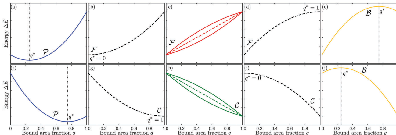
Fig. 4 Functional dependence of the local energy landscape \Delta\tilde{E} on the bound area fraction q with 0 \leq q \leq 1 , as described by eqn (46) for different values of the spontaneous curvature \bar{m} , the contact mean curvature \bar{M}_{co} , and the local mean curvature \bar{M} of the vesicle membrane. The upper panels (a–e) correspond to \bar{M}_{co} < \bar{m} , the lower panels (f–j) to \bar{m} < \bar{M}_{co} . In both rows of panels, the local mean curvature \bar{M} increases from left to right and the dashed energy functions represent marginal or degenerate cases: (a and f) landscapes for partially engulfed particles with a minimum at q_{eq} = q_{min}^* and 0 < q_{min}^* < 1 . The landscape in (a) illustrates the case with \bar{M} < \bar{M}_{co} < 2\bar{m} - \bar{M}_{co} and the one in (f) the case with \bar{M} < 2\bar{m} - \bar{M}_{co} < \bar{M}_{co} ; (b–d) landscapes for free or non-engulfed particles with a boundary minimum at q_{eq} = 0 . These landscapes are obtained for (b) \bar{M} = \bar{M}_{co} which defines the stability limit of the free state as described by eqn (12); (c) \bar{M}_{co} < \bar{M} < 2\bar{m} - \bar{M}_{co} ; and (d) \bar{M} = 2\bar{m} - \bar{M}_{co} corresponding to the stability limit of the completely engulfed state as in eqn (13) with \bar{M}' \approx \bar{M} . The linear landscape in (c) represents the degenerate case with \bar{M} = \bar{m} ; (g–i) landscapes for completely engulfed particles with a boundary minimum at q_{eq} = 1 . These landscapes are obtained for (g) \bar{M} = 2\bar{m} - \bar{M}_{co} corresponding to the stability limit of the completely engulfed state, (h) 2\bar{m} - \bar{M}_{co} < \bar{M} < \bar{M}_{co} , and (i) \bar{M} = \bar{M}_{co} which defines the stability limit of the free state. The linear landscape in (h) again represents the degenerate case with \bar{M} = \bar{m} ; (e and j) landscapes for bistable engulfment with an energy barrier at q_{ba} = q_{max}^* that is located between the two boundary minima at q = 0 and q = 1 . The landscape in (e) illustrates the case with \bar{M} > 2\bar{m} - \bar{M}_{co} > \bar{M}_{co} and the one in (j) the case with \bar{M} > \bar{M}_{co} > 2\bar{m} - \bar{M}_{co} . In all cases, \Delta E(q = 0) = 0 by definition.
