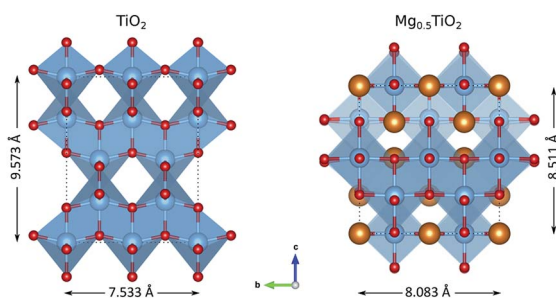
Fig. 7 Structural changes between \text{TiO}_2 and \text{Mg}_{0.5}\text{TiO}_2 , illustrated with a (2 \times 2 \times 1) unit cell. The \text{Mg}_{0.5}\text{TiO}_2 ordering shown is the most stable calculated (Fig. S13b†).
