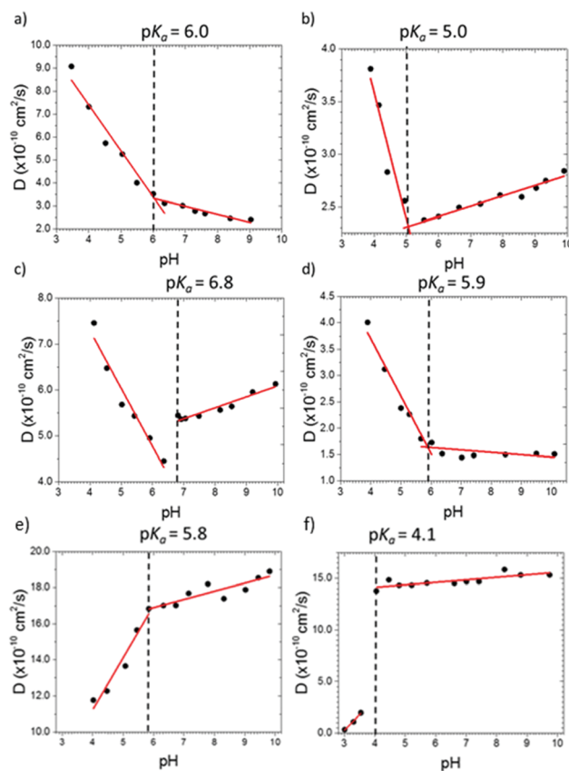
Fig. 4 Change in the diffusion coefficient of the TM as pH is lowered by the addition of HCl (0.1 M) in a solution (5 mg mL -1 ) of (a) 1 ; (b) 2 ; (c) 3 ; (d) 4 . The dashed line represents the apparent pK_a values for these gelators. (e and f) Show analogous data for (e) 5 (f) 10 , where no gel is formed when the pH is decreased.
