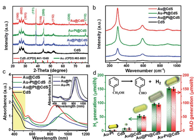
Fig. 2 (a) XRD patterns, (b) Raman spectra and (c) absorption spectra of CdS and metal–CdS hybrids. The inset of (c) shows the normalized absorption spectra of Au, Au@Pt and Au–Pt for comparison. (d) \text{H}_2 and benzaldehyde (BAD) generation rate in the photocatalytic conversion of benzyl alcohol (BA) under Vis-NIR light ( \lambda > 420 nm) irradiation over Au–Pt, CdS and metal–CdS hybrids. The insets of (d) show the formula for photocatalytic conversion of BA and the corresponding structural models of the samples.
