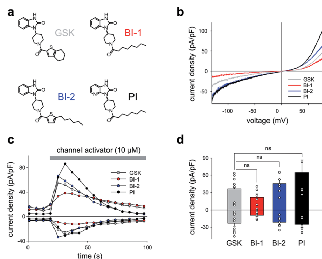
Fig. 1 (a) Chemical structures of GSK1702934A (GSK) and GSK derivatives (BI-1, BI-2 and PI). (b) Current to voltage relations of the net conductances ( I_{\max} - I_{\text{base}} ) induced by GSK, BI-1, BI-2 and PI (10 \mu\text{M} each) obtained in TRPC3-transfected HEK293 with voltage-ramp protocols. (c) Representative time courses of the TRPC3 conductances recorded at -90 mV and +70 mV during administration of channel activators (GSK, BI-1, BI-2 and PI as indicated) at 10 \mu\text{M} concentrations. (d) Current density of net, maximum responses obtained at -90 mV and +70 mV (mean \pm SEM). Statistical significance was tested by two tailed t -test (normally distributed values) or Mann-Whitney tests (non-normally distributed values). ns = not significant ( p > 0.05 ); N cells: GSK = 9; BI-1 = 6; BI-2 = 7; PI = 5.
