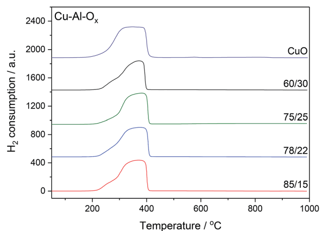
Fig. 3 H_2 -TPR profiles of Cu-Al- O_x mixed metal oxides; experimental conditions: mass of the catalysts = 30 mg; [H_2] = 5.0\text{ vol}\% , Ar balance, flow rate = 25\text{ cm}^3\text{ min}^{-1} , linear heating of 10\text{ }^\circ\text{C min}^{-1} .
