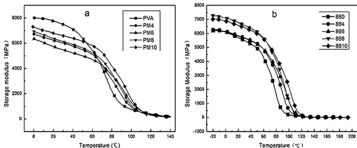
Fig. 8 Plots of storage modulus E' against temperature of PVA1799 (a) and PVA1788 (b) with various contents of \text{MgCl}_2 \cdot 6\text{H}_2\text{O} .
