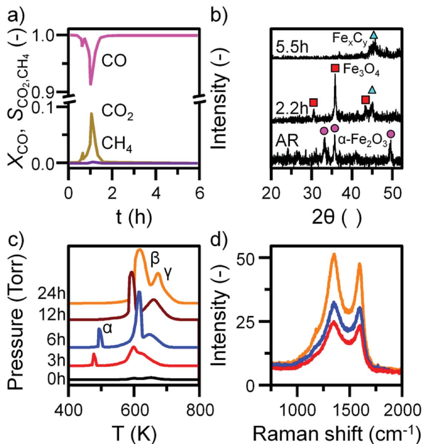
Fig. 1 (a) The conversion of CO and selectivity to \text{CO}_2 and \text{CH}_4 over the \alpha\text{-Fe}_2\text{O}_3 sample during CO hydrogenation at 623 K in the micro-reactor. (b) In situ XRD with identified reflections attributed to \alpha\text{-Fe}_2\text{O}_3 (circle), \text{Fe}_3\text{O}_4 (square), and iron carbides (triangle). (c) In situ TPO MS profiles and (d) selected ex situ Raman spectra of the \alpha\text{-Fe}_2\text{O}_3 sample after CO hydrogenation at 623 K in the micro-reactor. TPO profiles are stacked to facilitate comparison.
