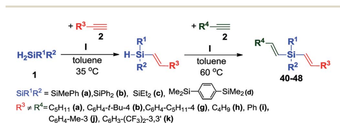
Scheme 6 Unsymmetrical bis-hydrosilylation.
