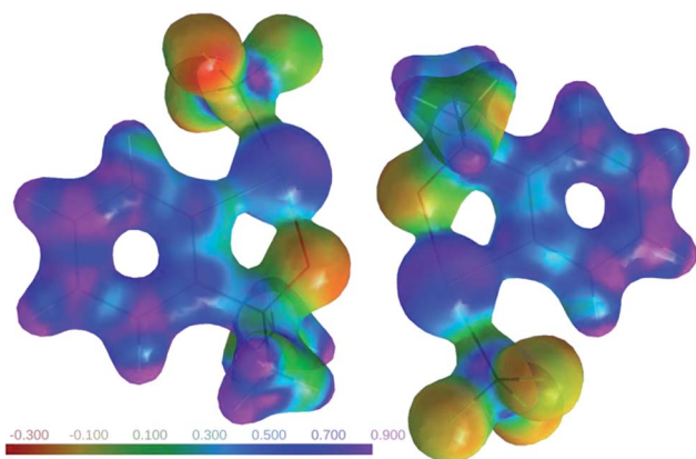
Fig. 5 Electrostatic potential for a pair of molecules in 1 mapped on an electron density isosurface ( \rho = 0.5e \text{ Å}^{-3} ; program MoleCoolQt 44,45 ).
