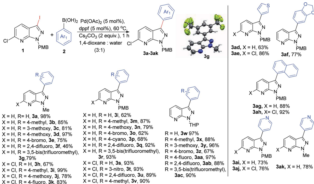
Scheme 1 Synthesis of C3-arylpyrazolo[3,4-b]pyridines and their derivatives. a, b Reaction conditions: 6-chloro-3-iodo-1-(4-methoxybenzyl)-1H-pyrazolo[3,4-b]pyridine (1.0 equiv.), arylboronic acid (1.0 equiv.), catalyst (5 mol%), dppf (5 mol%), base (2.0 equiv.), 1,4 dioxane : water (3 : 1) (5 mL), 60 °C, 1 h, air; b isolated yields.
