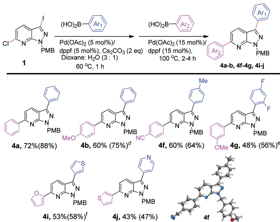
Scheme 3 Sequential one-pot synthesis of 3,6-diarylpyrazolo[3,4- b ]pyridines. a,b,c a Reaction conditions: 6-chloro-3-iodo-1-(4-methoxybenzyl)-1H-pyrazolo[3,4- b ]pyridine 1 (1.0 equiv.), arylboronic acid 2 (1.0 equiv.), Pd(OAc) 2 (5 mol%), dppf (5 mol%), Cs 2 CO 3 (2.0 equiv.), 1,4-dioxane : water (3 : 1) (5 mL), 60 °C for 1 h; after consumption of pyrazolopyridine 1 , addition of Pd(OAc) 2 (15 mol%), dppf (15 mol%), arylboronic acid 2 (1.2 equiv.), 100 °C, 2–4 h; b isolated yields; c formal average yields of the two steps shown in parentheses; d 10% of starting material recovered; e 6 h for second arylation and 15% of starting material recovered; f 6–8 h for second arylation.
