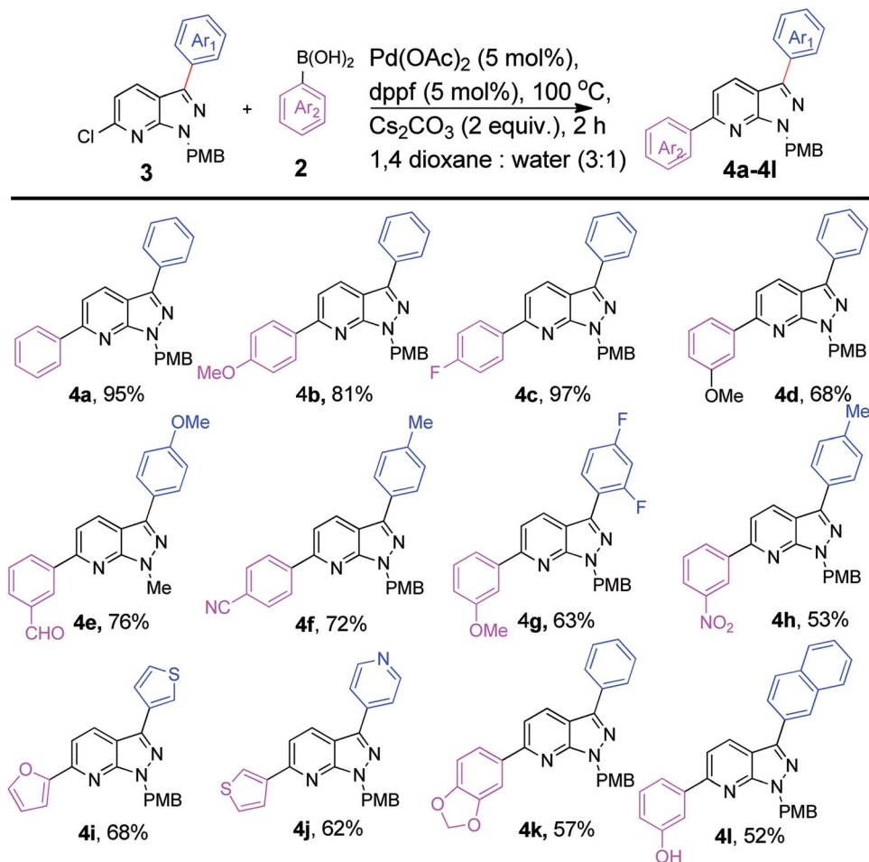
Scheme 2 Pd-catalyzed C6-arylation of 3-arylpyrazolo[3,4- b ]pyridines. a,b a Reaction conditions: 6-chloro-1-(4-methoxybenzyl)-3-phenyl-1H-pyrazolo[3,4- b ]pyridine 3 (1.0 equiv.), arylboronic acid 2 (1.0 equiv.), Pd(OAc) 2 (5 mol%), dppf (5 mol%), Cs 2 CO 3 (2.0 equiv.), 1,4-dioxane : water (3 : 1) (5 mL), 100 °C, 2 h; b isolated yields.
